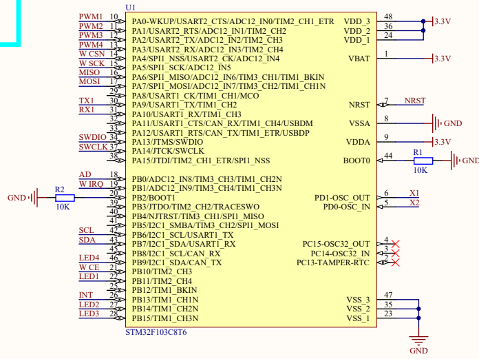
STM32F103C8T6
